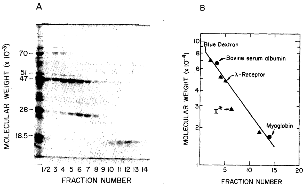
Fig.2. Gel chromatographic fractionation of HMPT-dissolved proteins on Sephacryl S-200. A column (59 x 1.5 cm) of Sephacryl S-200 was packed in a solvent mixture prepared by adding 500 mM Tris-SO 4 , 1 M LiCl, pH 7.5 (1 part) to HMPT (9 parts). This solvent mixture deposited some solid LiCl upon aging, and was used only after storage for 2 days. The sample (450 \mu l, see text) was layered onto the column bed. Fractions of 0.95 ml were collected at 25°C at a flow rate of about 2 ml/h. Due to a malfunction of the fraction collector, fractions 1 and 2 of the experiment shown were collected in one tube. A portion of each fraction (usually 12 \mu l; for fraction 1/2 4 \mu l) was added to 50 \mu l SDS- \beta -mercaptoethanol sample buffer [11]. After heating (15 min, 100°C), 20 \mu l portions of these samples were analyzed by SDS-polyacrylamide slab gel electrophoresis (fig.2A). The protein profile of the sample applied to the column is shown in the left lane of fig.2A. The calibration of the SDS-gels with known marker proteins allowed us to assign molecular weights to the major polypeptide components of the HMPT extract. These molecular weights were then plotted on semi-logarithmic paper against the fraction number where maximal elution occurred (fig.2B, \blacktriangle ). The elution positions ( \bullet ) for bovine serum albumin and myoglobin were determined in independent experiments.
